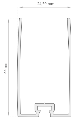
Expansor D-2018
