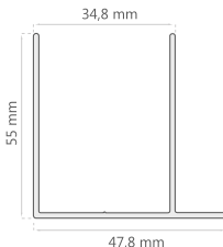
Expansor D-2055
